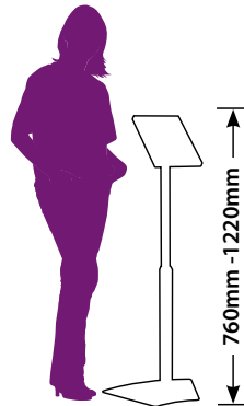
Footprint: 440 [w] x 345 [d]mm
