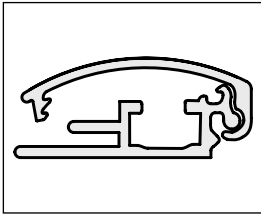
25mm profile with mitred corners.
